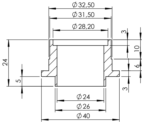
S.s cylinder bushing Cod. 204640
