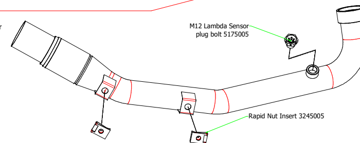
73011KZ Catalytic Homologated Collector
