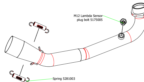
53046MI Racing Collector
